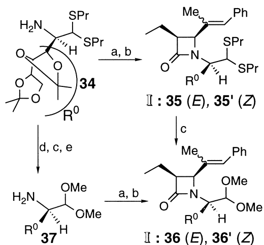
Scheme 3. Reagents: (a) \text{PhCH}=\text{C}(\text{Me})\text{CHO} , toluene, reflux; (b) TEA, \text{CH}_3(\text{CH}_2)_2\text{COCl} , toluene, reflux; (c) \text{PhI}(\text{COCF}_3)_2 , MeOH, rt; (d) CBZ, MeOH, \text{Na}_2\text{CO}_3 , rt; (e) \text{H}_2/\text{Pd-C}(5\%) , EtOH, rt.
