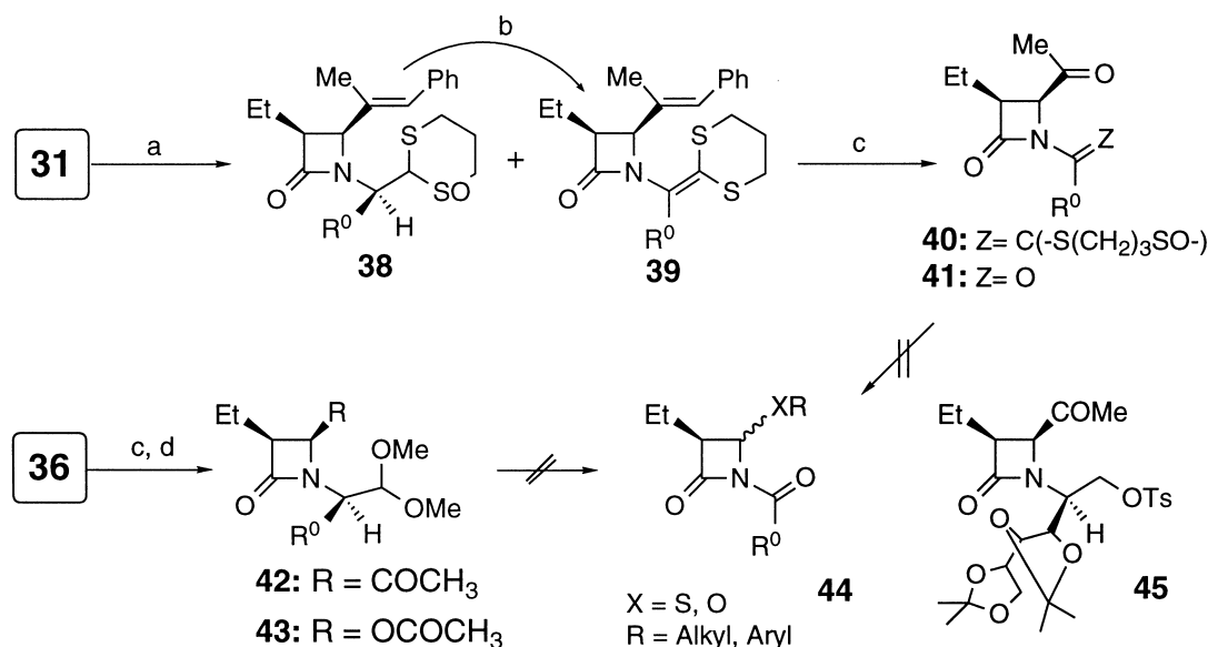
Scheme 4. Reagents: (a) PhICl 2 , CH 2 Cl 2 , -40 °C; (b) O 3 , CH 2 Cl 2 , -78 °C; Me 2 S, rt; (c) m -CPBA, CH 2 Cl 2 , rt.
