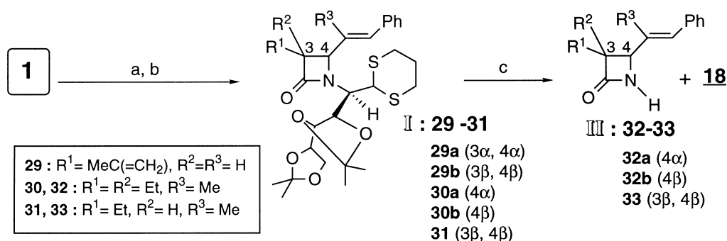
Scheme 2. Reagents: (a) \text{PhCH}=\text{C}(\text{R}^3)\text{CHO} , toluene, reflux; (b) TEA, \text{R}^1\text{R}^2\text{CHCOCl} , toluene (or \text{CH}_2\text{Cl}_2 ), reflux; (c) n\text{-BuLi} , THF, -40^\circ\text{C} .
